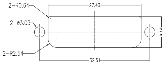
Panel Cutout
