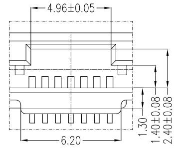
VIEW 0 SCALE 3:1
