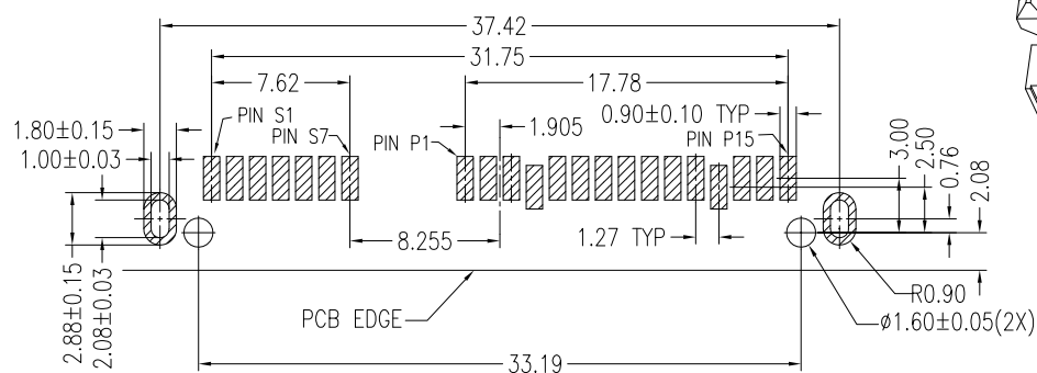
PCB LAYOUT(T=1.20mm) COMPONENT SIDE
