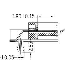
SECT B-B
