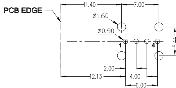
RECOMMEND PCB LAYOUT TOP VIEW
