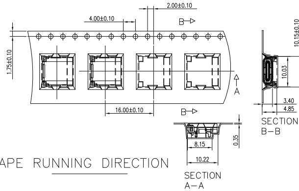
USB C TYPE 24pin SMT Connector
